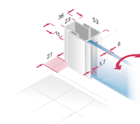
Door panel closing side
