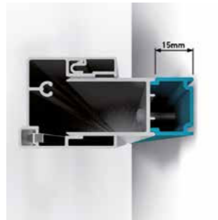
Enlargement profile 508838
