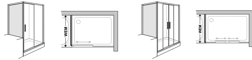
View, hinged left
