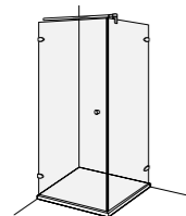
View, hinged left
