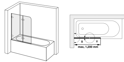
View, hinged left
